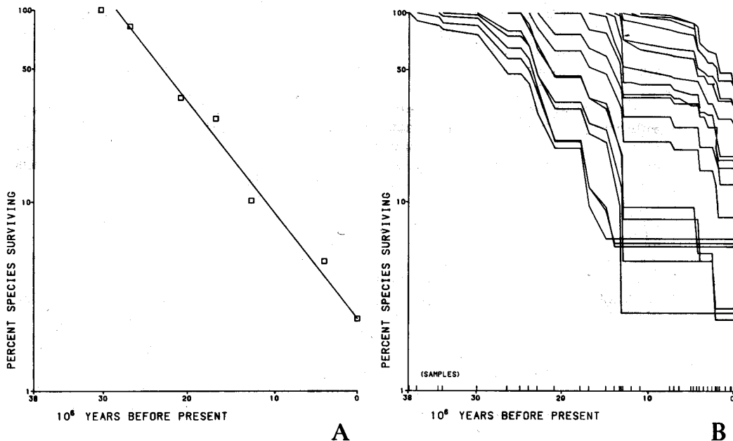
TEXT-FIG. 4. A, survivorship pattern for a polycohort of planktonic foraminiferal species from 30 ma BP (Early Oligocene) to the present, sampled at intervals of approximately 5 ma. The fitted straight line implies continuous, background extinction following Van Valen's Law. (From Raup 1986; data from Hoffman and Kitchell 1984.) B, survivorship patterns for a set of polycohorts of planktonic foraminiferal species from 30 ma BP to the present. Sampling points are shown on the inside of the lower, horizontal axis. The data points for survivorship have been connected by straight-line segments. This method of plotting emphasizes the episodic pattern of extinction in contrast to the method used in A. (From Raup 1986; redrawn from Hoffman and Kitchell 1984.)
