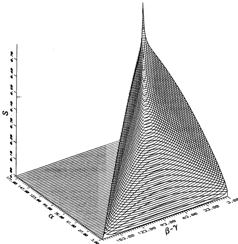
TEXT-FIG. 5. Surface obtained by plotting the values of S between 3^\circ < \alpha < 177^\circ and 3^\circ < \beta - \gamma < 177^\circ , for a constant value b_1/b_{1r} = 0.05 . The side facing the reader should be seen as concave.
