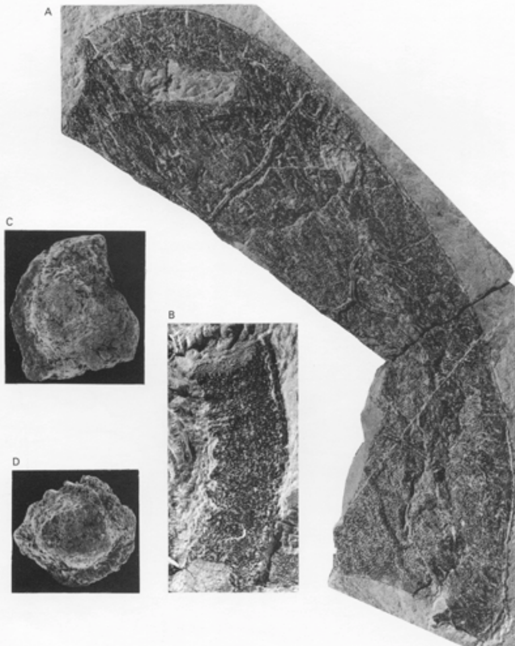
TEXT-FIG. 3. Bannhuanaspis vukhuci gen. et sp. nov. Lower Devonian (Late Lochkovian to Early Pragian), top part of Si Ka Formation or base of the Bac Bun Formation; Ban Nhuan, Phu Luong District, Bac Thai Province, Vietnam. A, Incomplete head shield (holotype, VND 50), exoskeleton in ventral view (for interpretation see Text-fig. 2A), \times 1 . B, fragment of ventral rim of head shield (VND 52), showing branchial notches, (for interpretation see Text-fig. 5A), \times 1 . C-D, isolated scales of the body squamation, associated with the holotype; scanning electron micrographs of the external surface, \times 50 .
